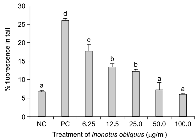
Fig. 4. The protective effect of supplementation in vitro with different concentration of EtOH extract of Inonotus obliquus on 200 \mu\text{M} \text{H}_2\text{O}_2 -induced human lymphocytes DNA damage. Values are mean with standard error of duplicate experiments with lymphocytes from each of two different donors. a~d Values not sharing same letters are significantly different from one another ( p < 0.05 ). NC: negative control (DMSO 1%), PC: positive control (200 \mu\text{M} \text{H}_2\text{O}_2 ).
