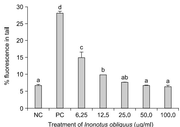
Fig. 5. The effect of supplementation in vitro with different concentration of EtOH extract of Inonotus obliquus and 200 \mu\text{M} \text{H}_2\text{O}_2 simultaneously in human lymphocytes. Values are mean with standard error of duplicate experiments with lymphocytes from each of two different donors. a~d Values not sharing same letters are significantly different from one another ( p < 0.05 ). NC: negative control (DMSO 1%), PC: positive control (200 \mu\text{M} \text{H}_2\text{O}_2 ).
