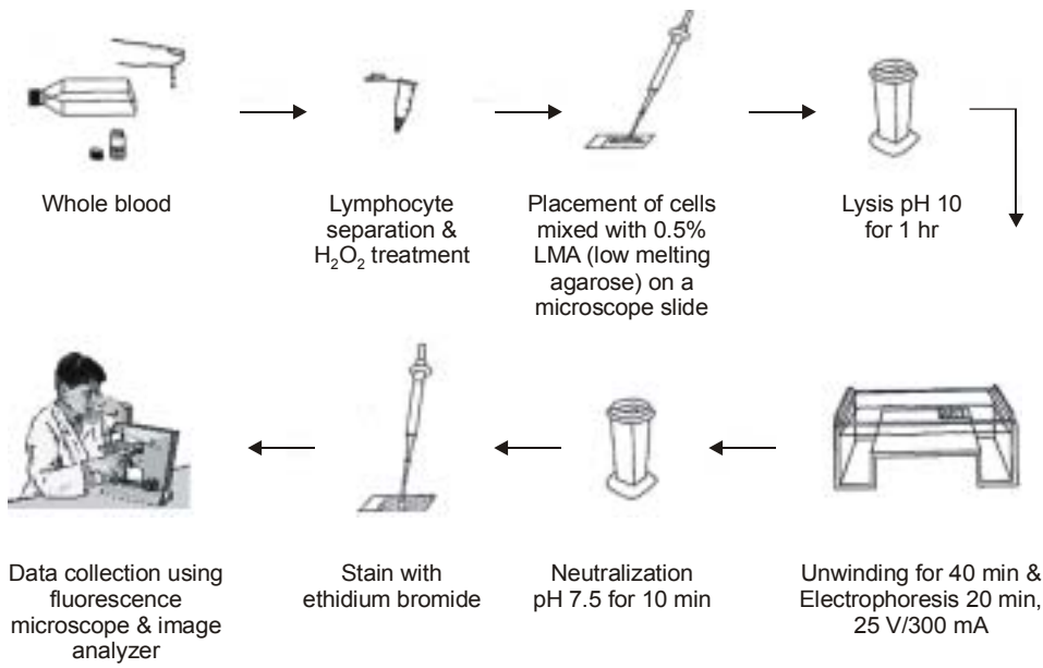
Fig. 1. Alkaline comet assay scheme.
