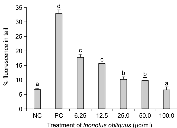
Fig. 3. The preventive effect of supplementation in vitro with different concentration of EtOH extract of Inonotus obliquus on 200 \mu\text{M} \text{H}_2\text{O}_2 -induced human lymphocytes DNA damage. Values are mean with standard error of duplicate experiments with lymphocytes from each of two different donors. a~d Values not sharing same letters are significantly different from one another ( p < 0.05 ). NC: negative control (DMSO 1%), PC: positive control (200 \mu\text{M} \text{H}_2\text{O}_2 ).
