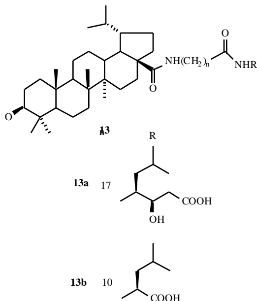
Fig. (5). C 17 derivatives of betulinic acid with potent anti-HIV activity.
