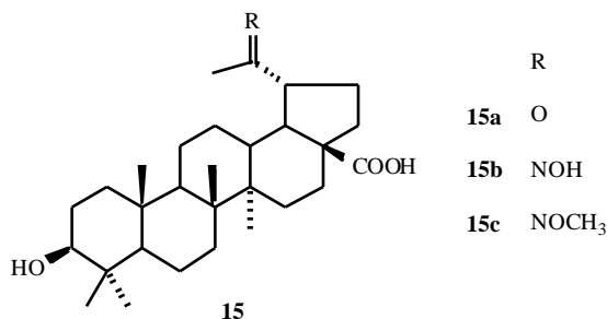
Fig. (7). \text{C}_{20} modified betulinic acid derivatives.
