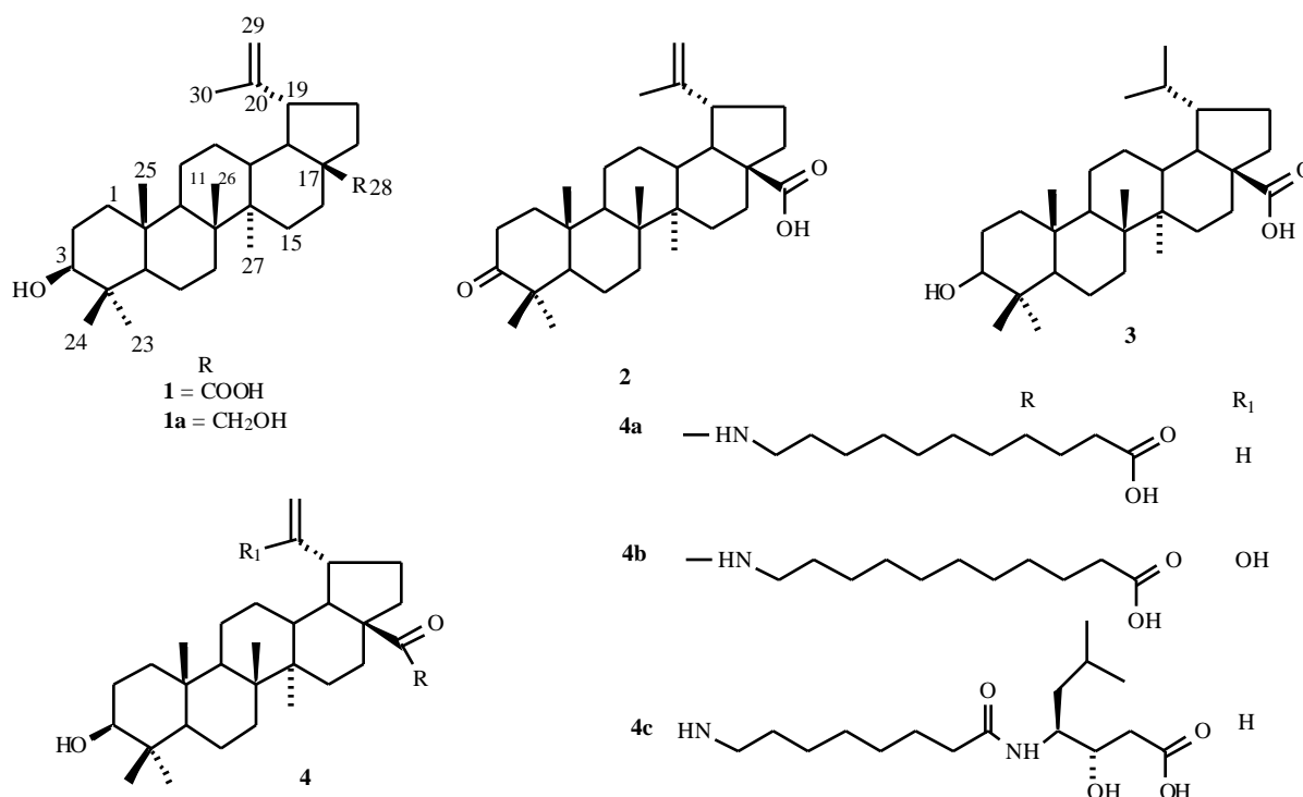
Fig. (1). Structures of betulinic acid, betulin, dihydrobetulinic acid and amide derivatives of betulinic acid.
