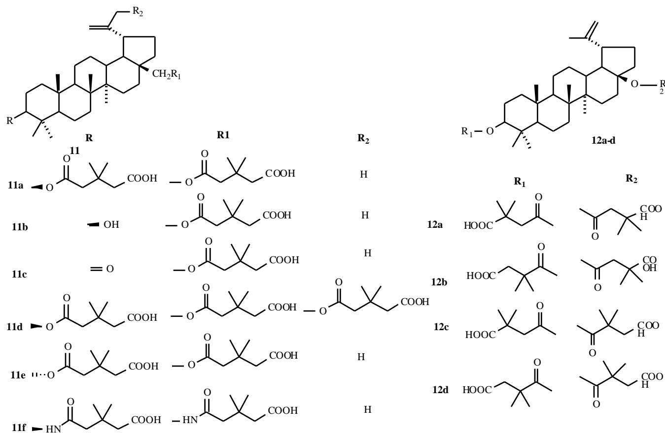
Fig. (4). O-acyl derivatives of betulinic acid and dihydrobetulinic acid.
