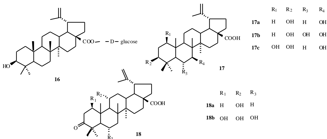
Fig. (8). Microbial biotransformation products of betulinic acid.
