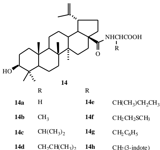
Fig. (6). \text{C}_{28} peptide derivatives of betulinic acid.
