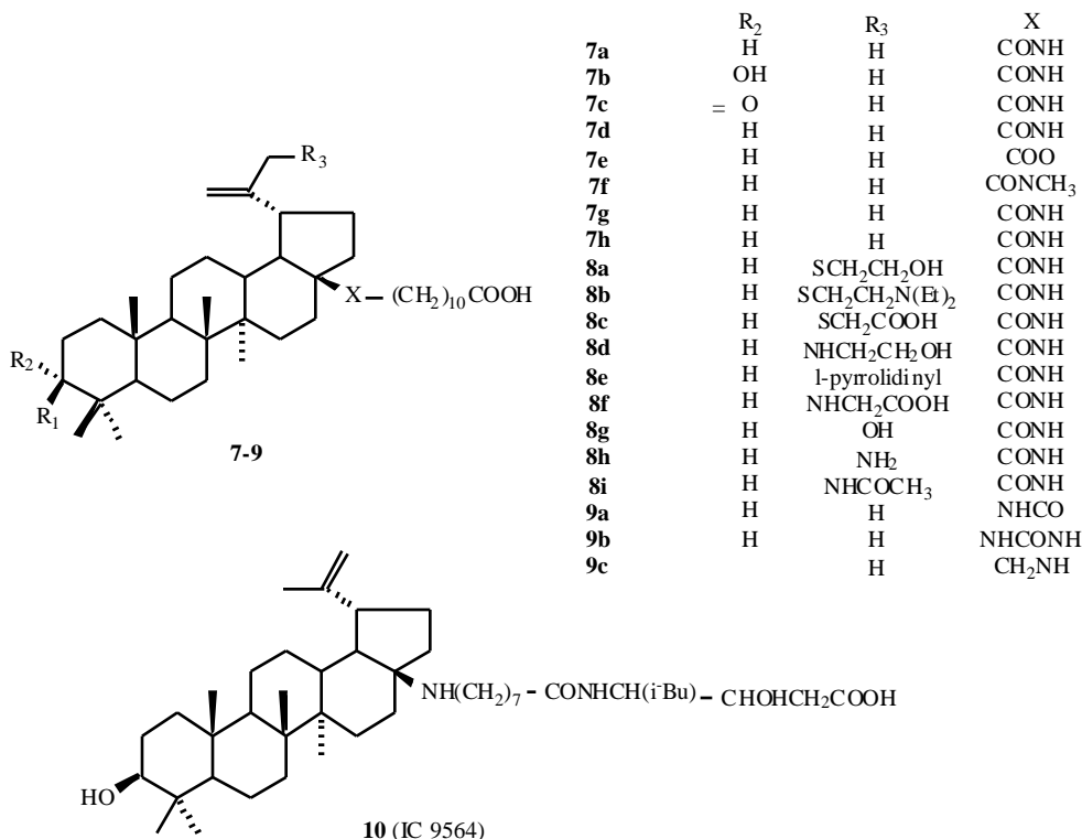
Fig. (3). C 17 modified betulinic acid derivatives.
