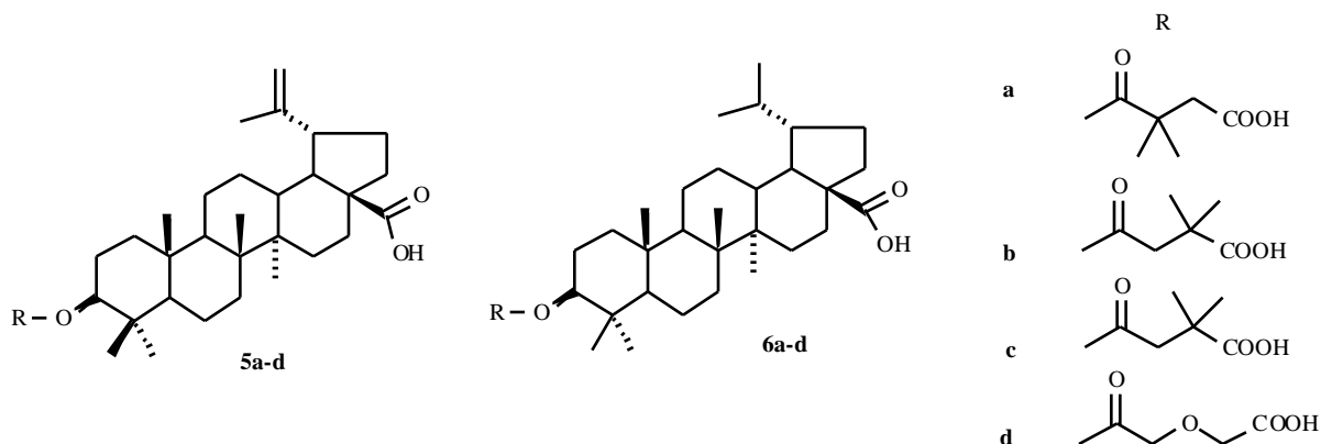
Fig. (2). C 3 modified derivatives of betulinic acid and dihydrobetulinic acid.
